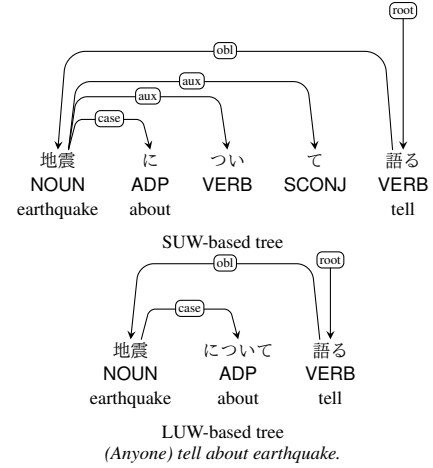
Figure 5: Multi-Word Expression
